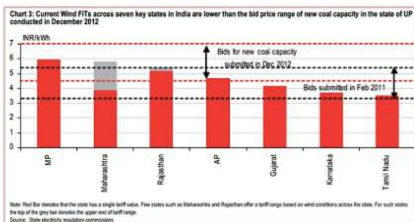
Figure 6: Wind Feed-in-Tariffs in India are below coal tariffs
